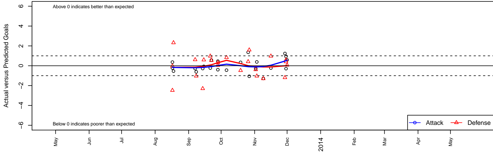
Arsenal FC West G02 Dots are actual minus expected GF (blue circles) and GA (red triangles). Blue line is smoothed change in attack strength. Red is smoothed change in defense strength.
